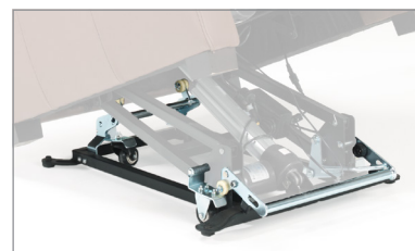
A - Trolley with castors 50 mm
